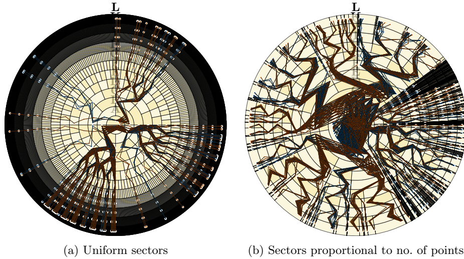
Fig. 6: Tsunami (12-dimensional) Dataset with 2 labels - RAYS Visualisation.
