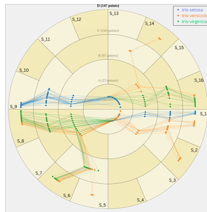
Fig. 1: Iris Dataset with 3 labels - RAYS Visualisation
